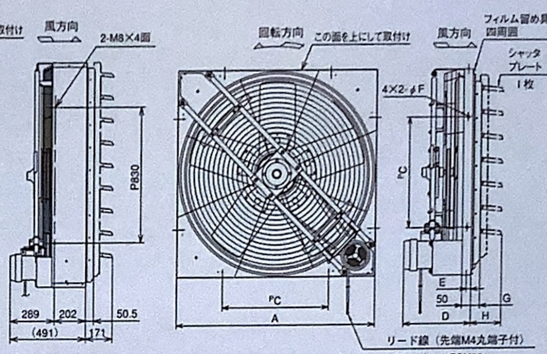
FGX621~1070
